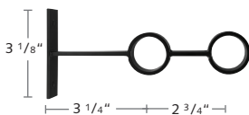
2230DCY-XX York Double Closed Bracket
