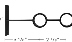
2220DCY-XX York Double Closed Bracket
